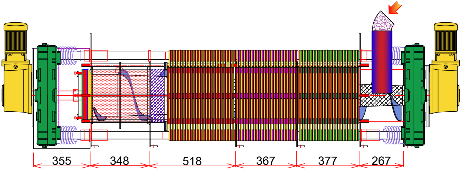
LEFT VIEW
