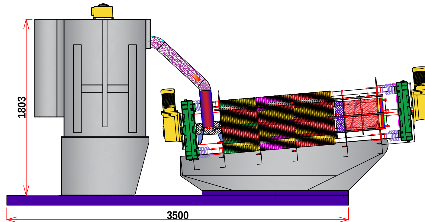
FRONT VIEW
