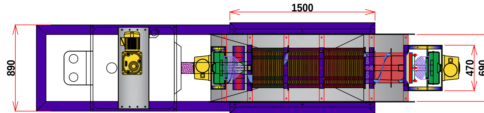
TOP VIEW
